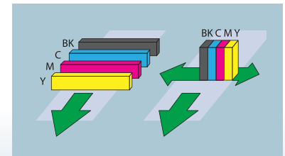
Single-pass printing SCL-4000 Serial printing
